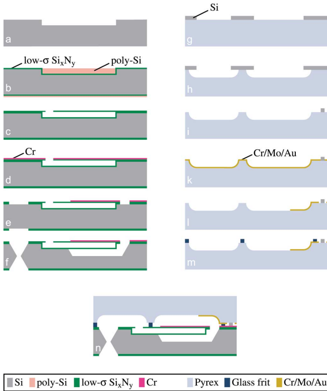
Fig. 3. Fabrication and packaging process: Suspended microchannels with a 1- \mu\text{m} fluid layer and 800-nm-thick silicon nitride walls are fabricated using a sacrificial polysilicon process and chemical mechanical polishing. Following the release, the device wafer is glass frit-bonded under vacuum to a Pyrex capping wafer.
