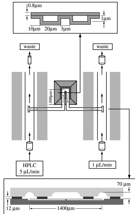
Fig. 7. Microfluidic bypasses enable the quick exchange of samples inside the suspended microchannel. The flow rate through the resonator is controlled by the pressure difference between the inlet and the outlet bypass.
